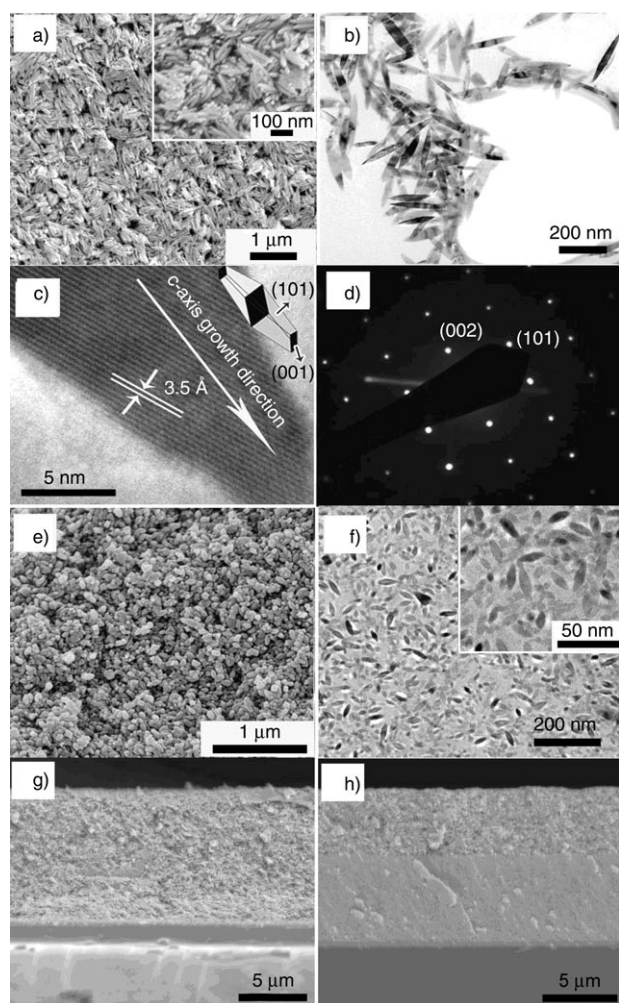
Figure 1. a, b) SEM and TEM images of the as-prepared large \text{TiO}_2 nanospindles. c, d) HRTEM image and the corresponding SAED pattern of a typical nanospindle. e, f) SEM and TEM images of the as-prepared small \text{TiO}_2 nanospindles. Cross-sectional SEM images for a single mesoscopic \text{TiO}_2 layer prepared from large nanospindles (g) and a double-layer structure from large and small nanospindles (h). Inset of a): Enlarged SEM image showing the close packing of large \text{TiO}_2 nanospindle bundles. Inset of c): Schematic illustration of the anatase crystal planes of \text{TiO}_2 nanospindles. Inset of f): Enlarged TEM image of the as-prepared small \text{TiO}_2 nanospindles.
